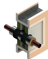
Thermally Lagged Copper Pipe Protected by Intustrap ® in a Fire Rated Plasterboard Wall
